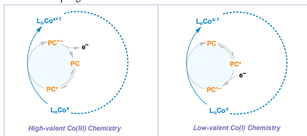
Figure 1. General schematic presentation of dual cobalt/photoredox strategies
