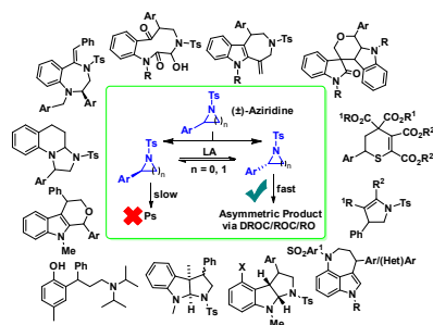
Scheme 1. Synthetic exploration of small ring Aza/oxa-heterocycles via DKR.
