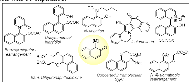
Scheme 1: Synthetic strategies using quinoid carbene
