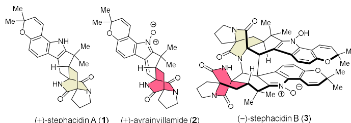
Figure. Architecturally intriguing secondary metabolites of biological relevance.
