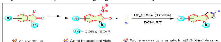
Figure 1. Rh(II)-catalyzed construction of furo[2,3-b]indole framework from isatin derived diazooxindoles and arylacetylenes
