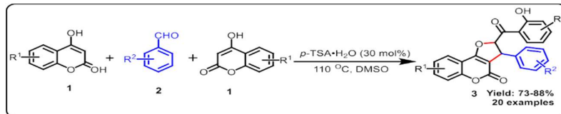
Scheme 1. Synthesis of dihydrofuro[3,2- c ]chromenone derivatives
