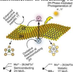
Figure. SET and energy transfer mechanisms governing TMDs photo-mediated catalytic processes.
