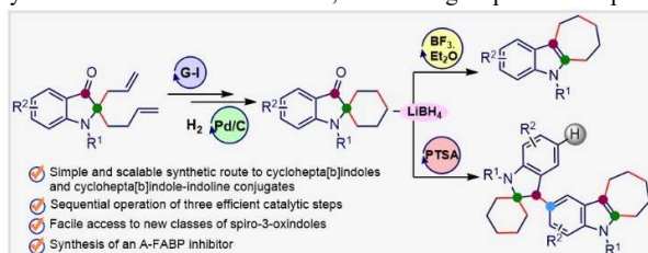
Scheme1: Synthesis of cyclohepta[b]indoles and cyclohepta[b]indole-indoline conjugates
