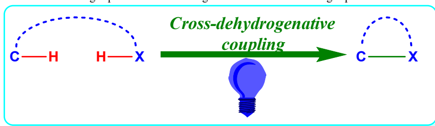
Scheme 1: Visible-Light-Promoted Cross-Dehydrogenative Coupling.
