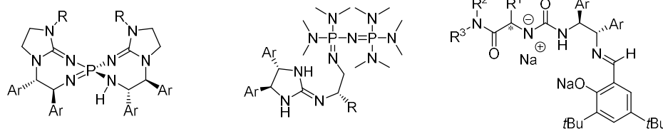
bis(guanidino)iminophosphorane catalyst ( M )- 1 cooperative binary base catalyst 2 ureate having phenoxide and Schiff base units 3
